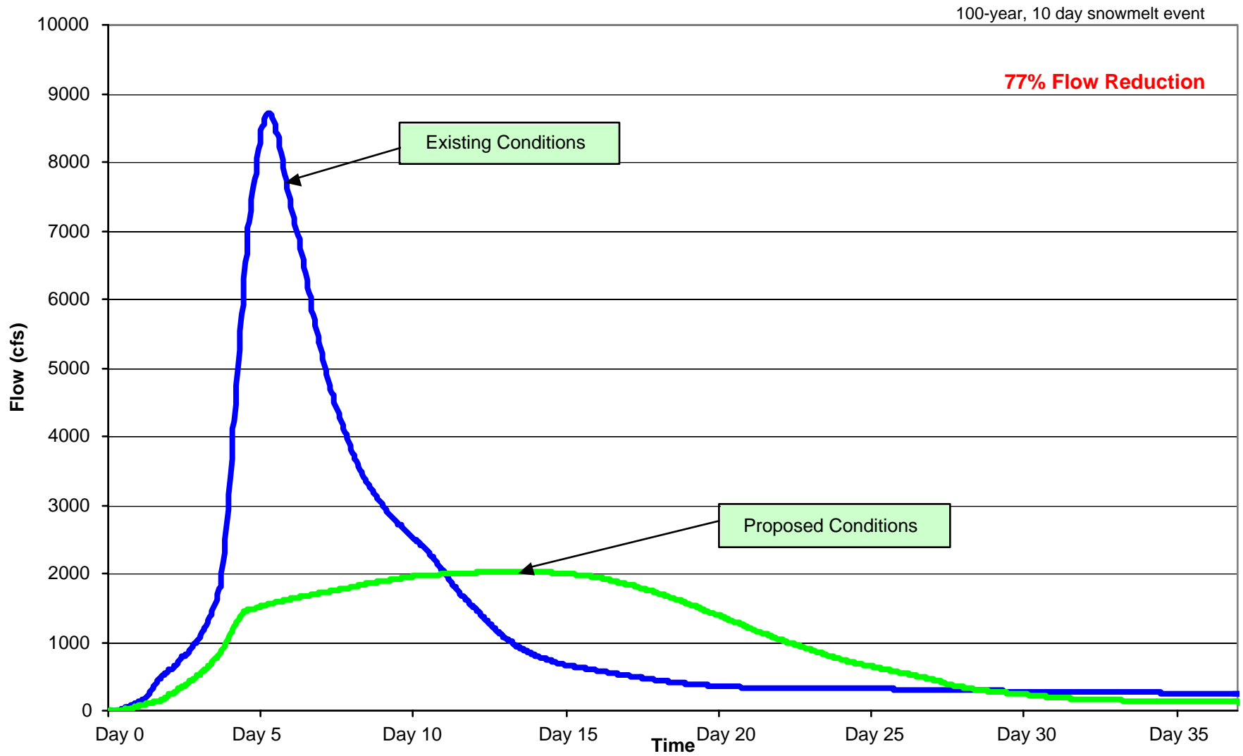
Figure 4a - Big Sioux River Headwaters Outlet, Reduction in Flow Rate
