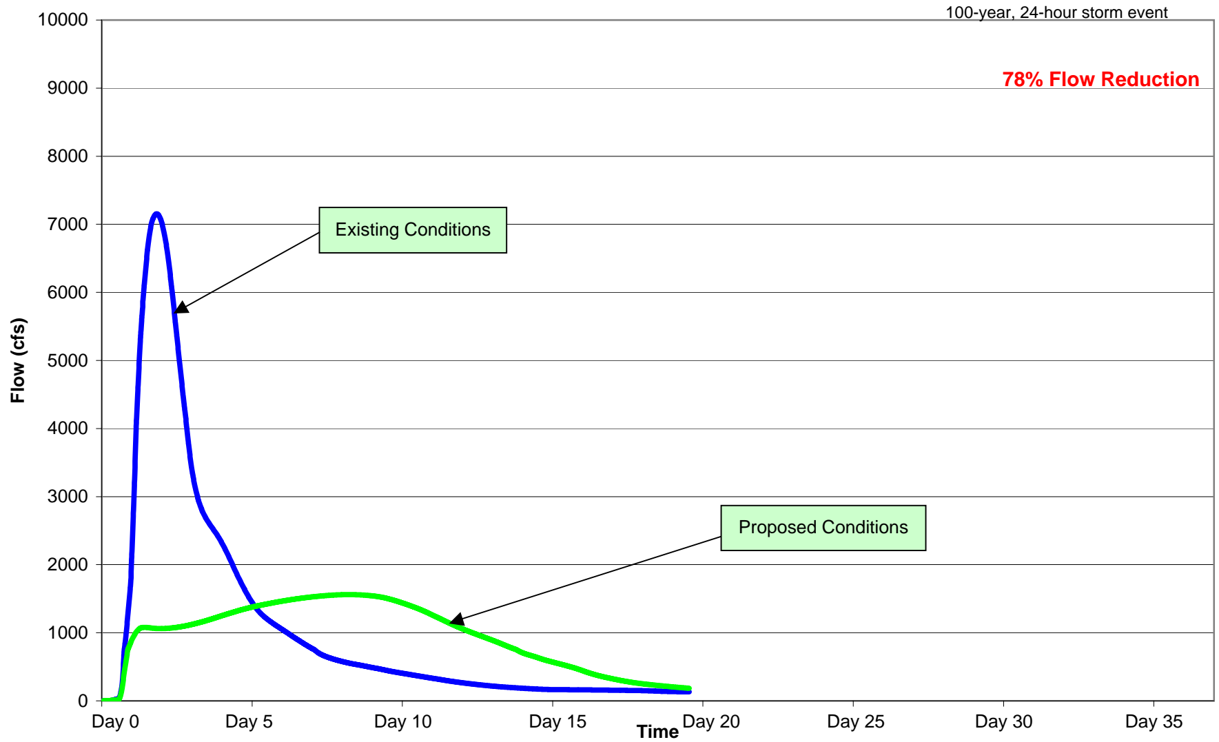
Figure 4b - Big Sioux River Headwaters Outlet, Reduction in Flow Rate
